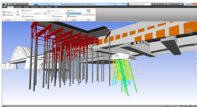
3D clash controls for new and existing foundations. Image courtesy of iNFRANEA.
