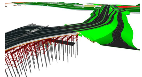
3D and 4D interface management for all temporary works. Image courtesy of iNFRANEA.
